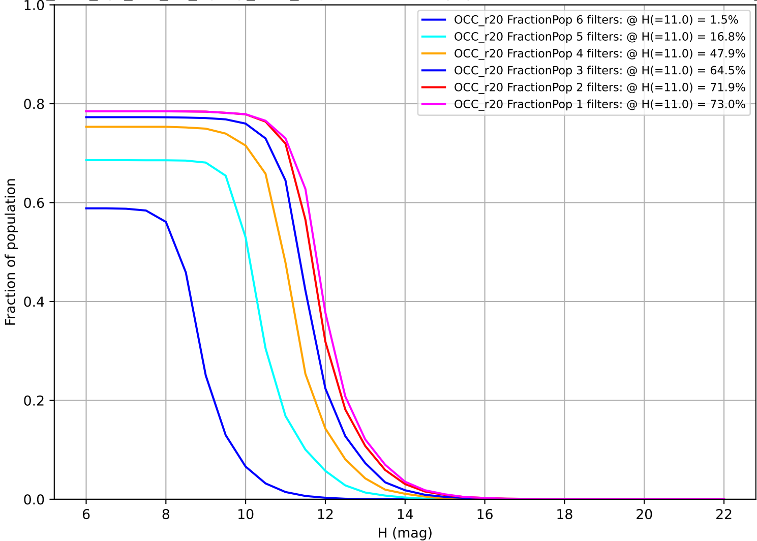
too_elab_2yr_r64_d2_ugrizy_v3.4_10yrs: Fraction of population with colors in X filters OCC_r20
