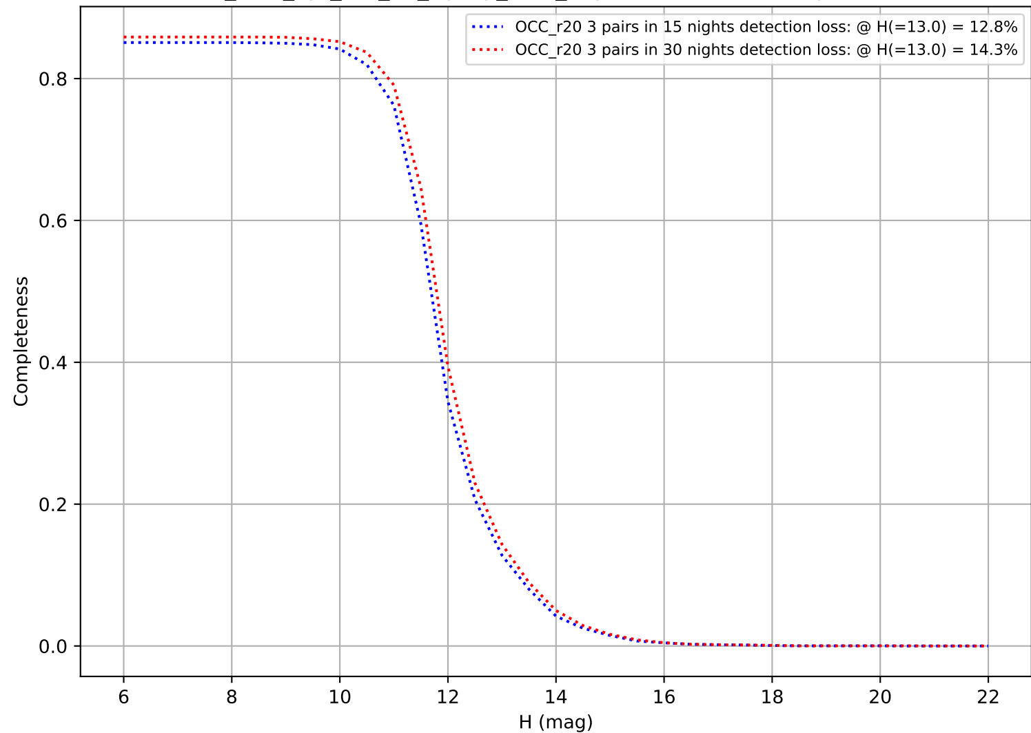
too_elab_2yr_r64_d2_ugrizy_v3.4_10yrs: DifferentialCompleteness
