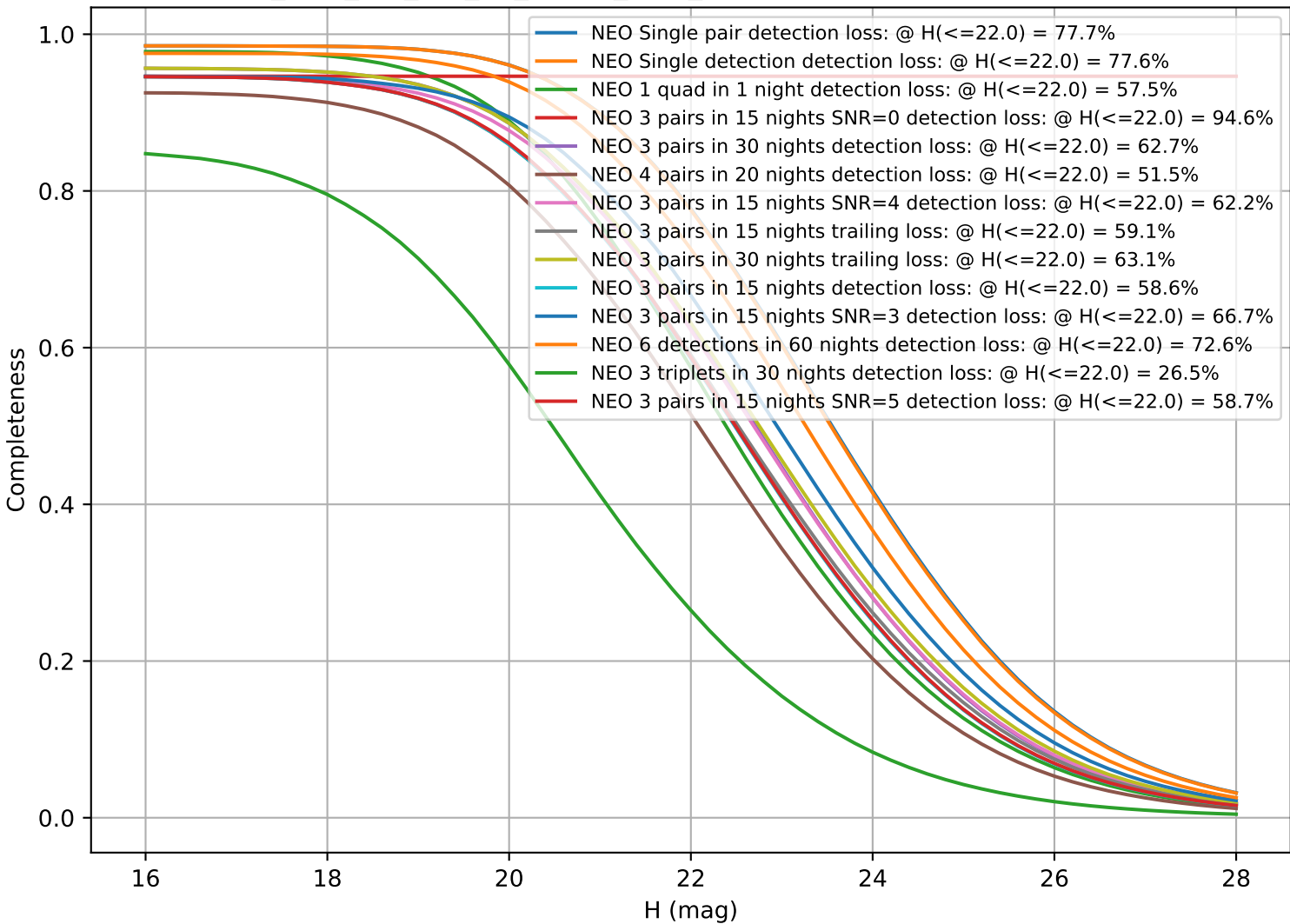
too_elab_2yr_r64_d2_ugrizy_v3.4_10yrs: CumulativeCompleteness
