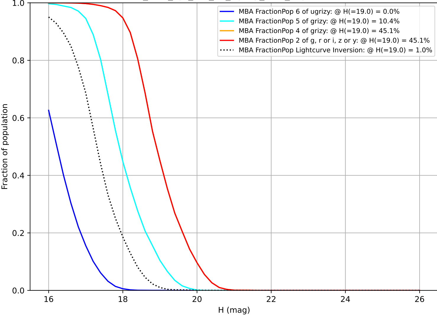
too_elab_2yr_r64_d2_ugrizy_v3.4_10yrs MBA
