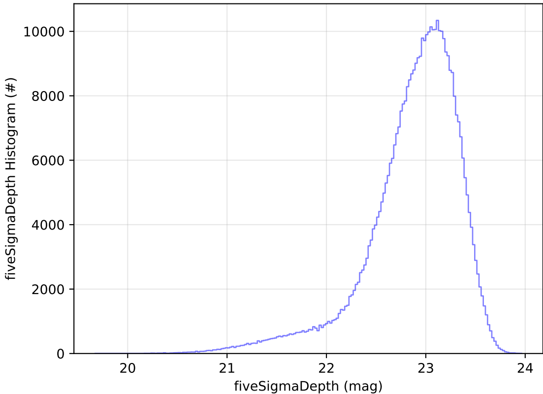
too_elab_2yr_r64_d2_ugrizy_v3.4_10yrs z: fiveSigmaDepth Histogram
