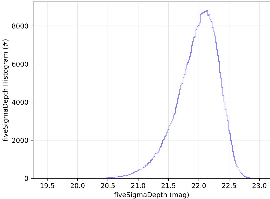
too_elab_2yr_r64_d2_ugrizy_v3.4_10yrs y: fiveSigmaDepth Histogram
