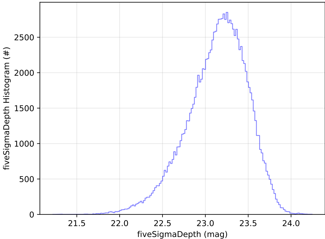
too_elab_2yr_r64_d2_ugrizy_v3.4_10yrs u: fiveSigmaDepth Histogram
