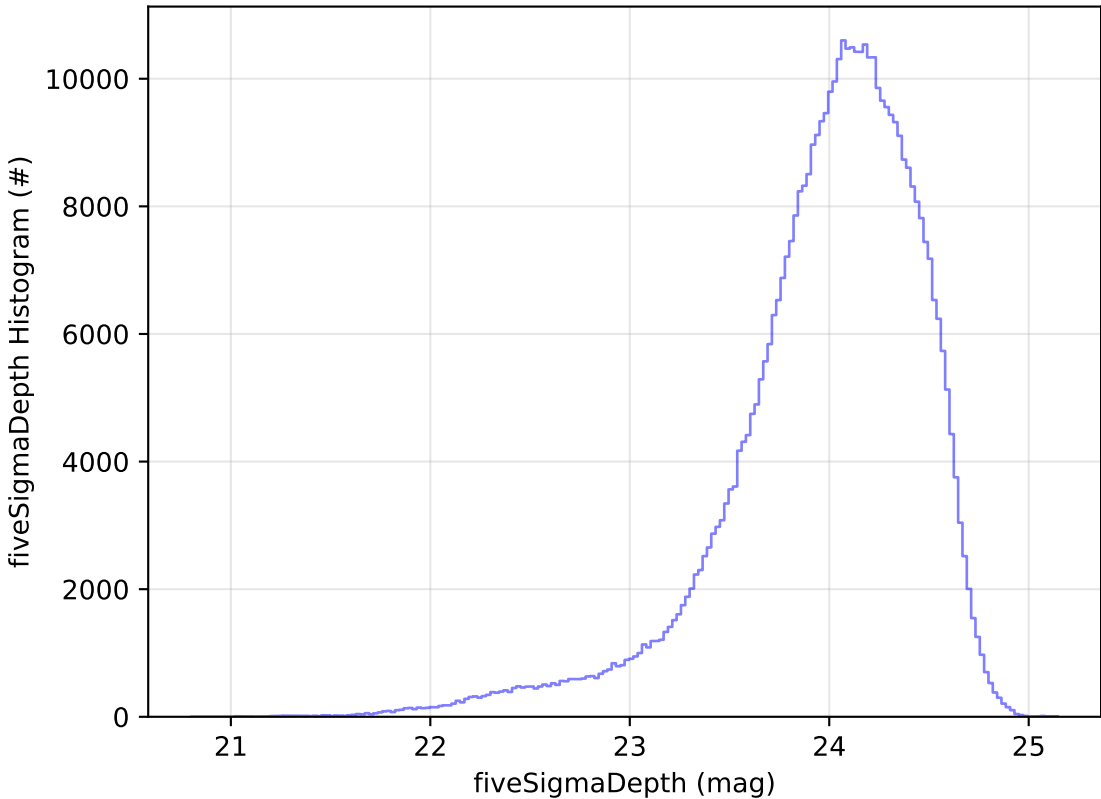
too_elab_2yr_r64_d2_ugrizy_v3.4_10yrs r: fiveSigmaDepth Histogram
