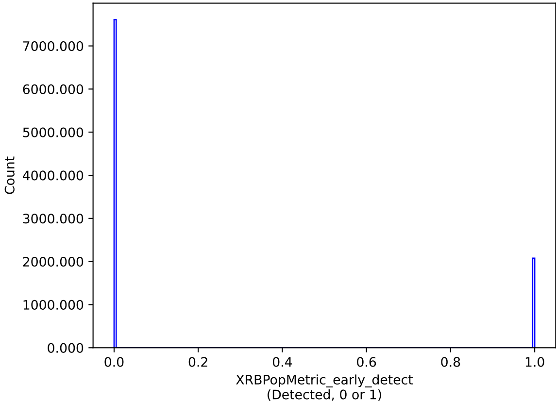
too_elab_2yr_r64_d2_ugrizy_v3.4_10yrs : XRBPoMetric_early_detect
