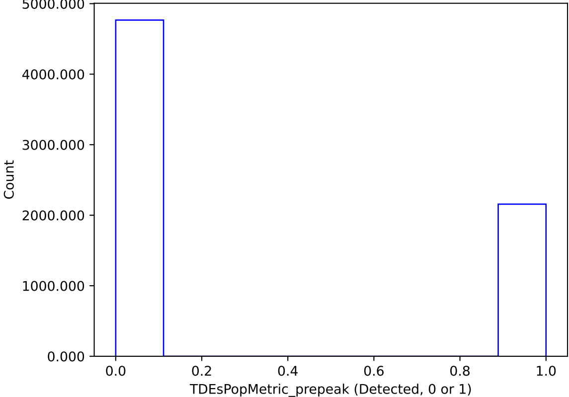
too_elab_2yr_r64_d2_ugrizy_v3.4_10yrs : TDEsPopMetric_prepeak
