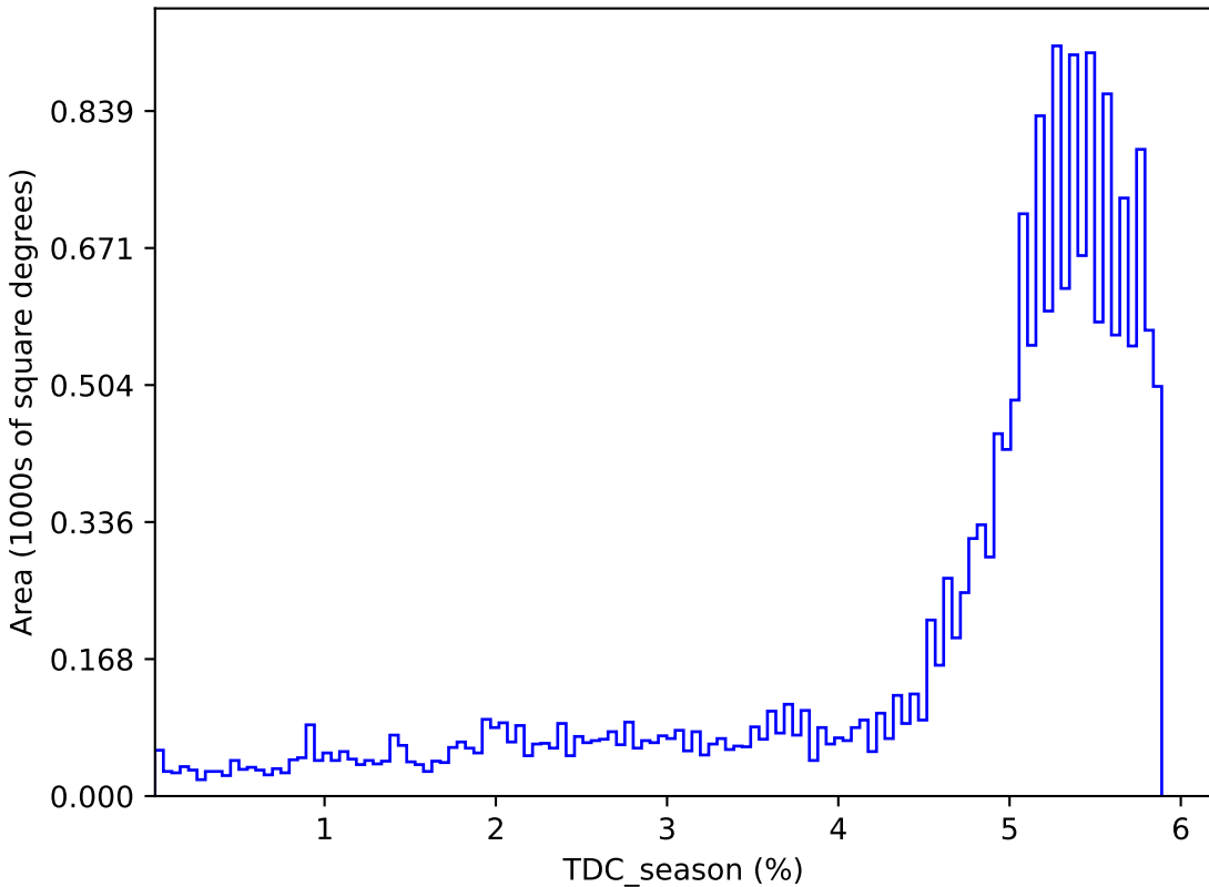
too_elab_2yr_r64_d2_ugrizy_v3.4_10yrs : TDC_season
