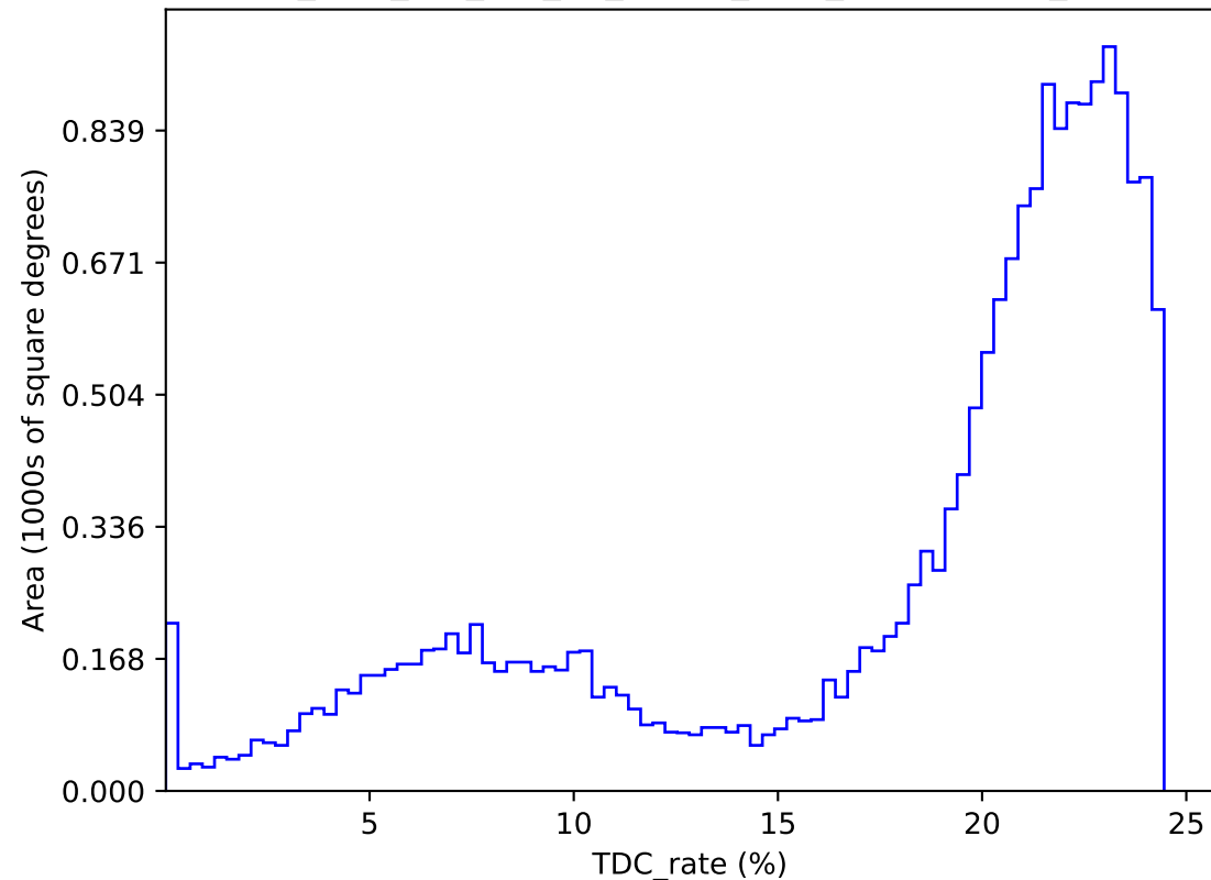
too_elab_2yr_r64_d2_ugrizy_v3.4_10yrs : TDC_rate
