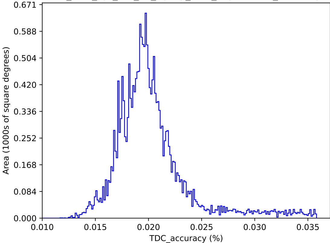
too_elab_2yr_r64_d2_ugrizy_v3.4_10yrs : TDC_accuracy
