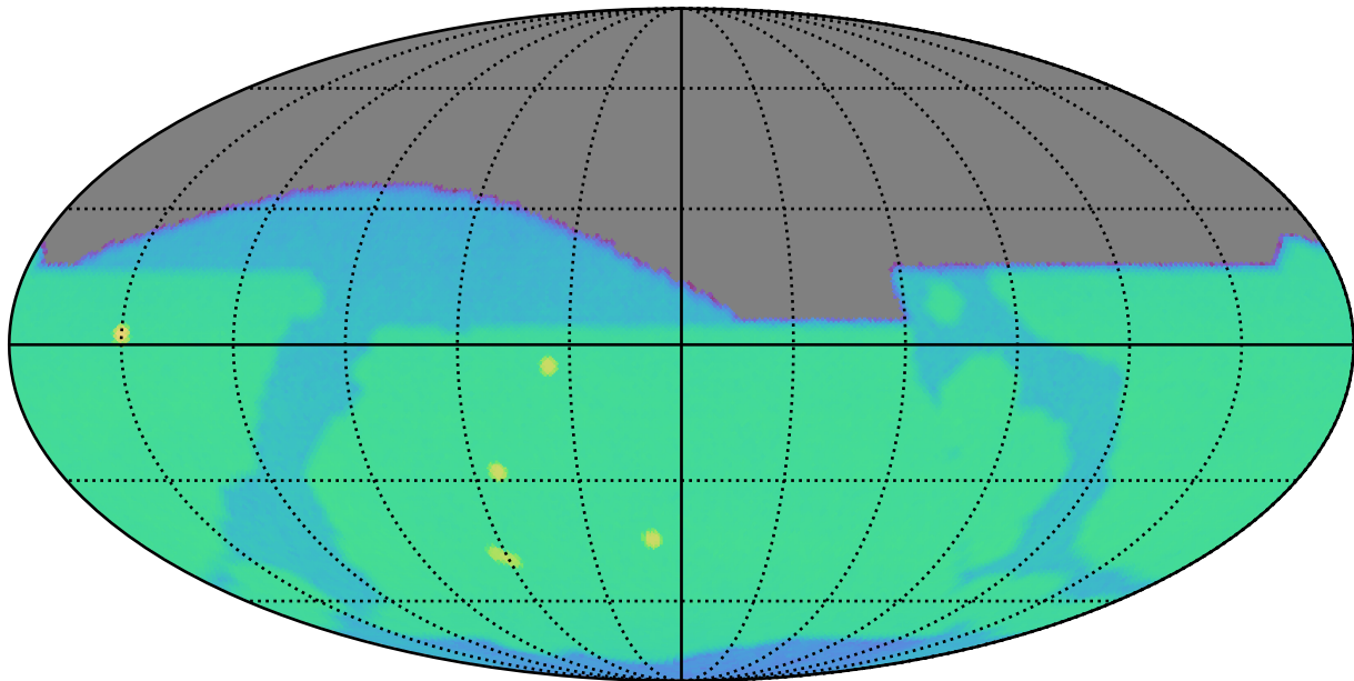
too_elab_2yr_r64_d2_ugrizy_v3.4_10yrs i: SurfaceBrightLimit
