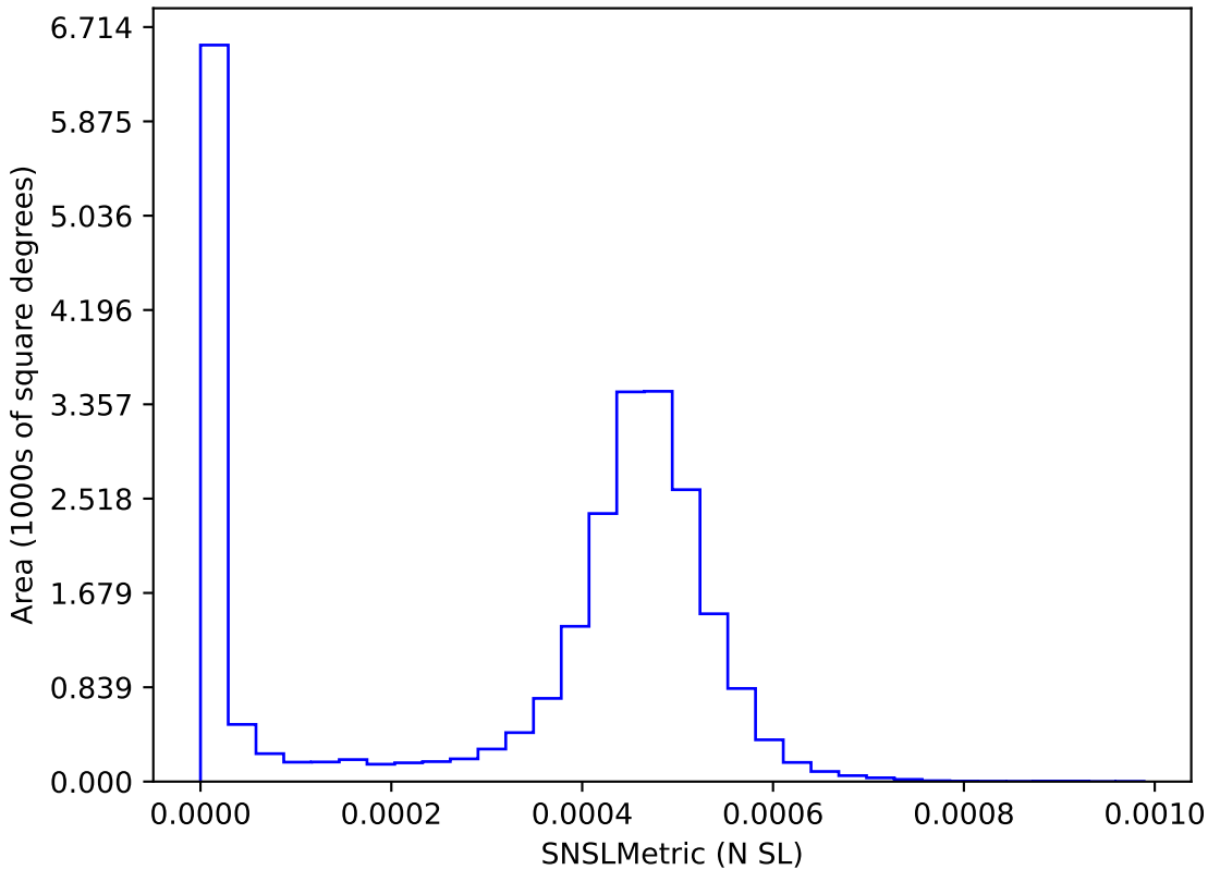
too_elab_2yr_r64_d2_ugrizy_v3.4_10yrs : SNSLMetric
