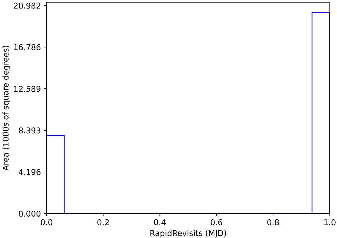
too_elab_2yr_r64_d2_ugrizy_v3.4_10yrs : RapidRevisits
