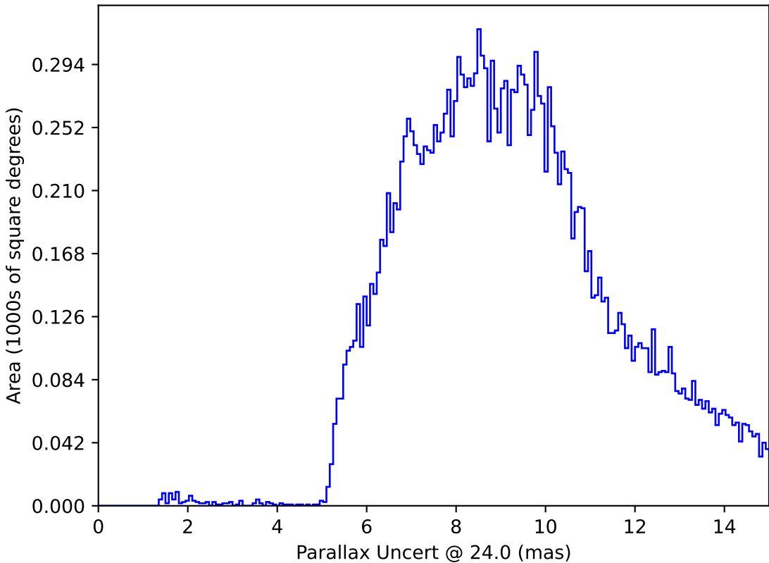
too_elab_2yr_r64_d2_ugrizy_v3.4_10yrs : Parallax Uncert @ 24.0
