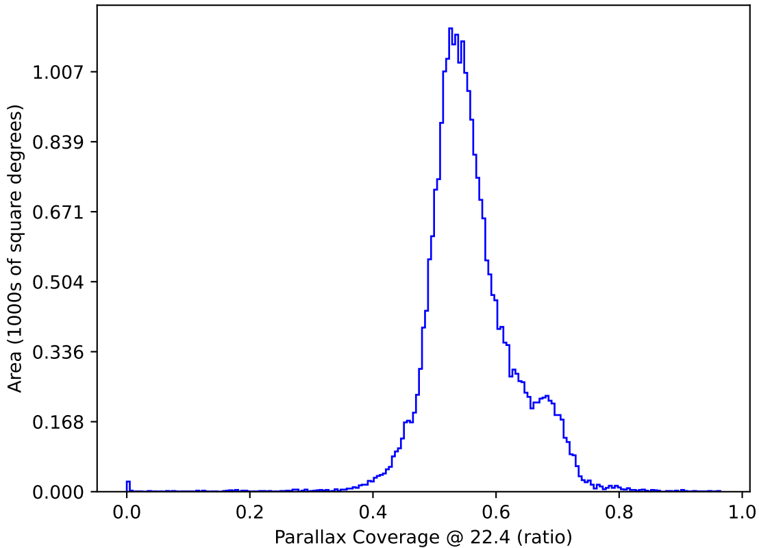
too_elab_2yr_r64_d2_ugrizy_v3.4_10yrs : Parallax Coverage @ 22.4
