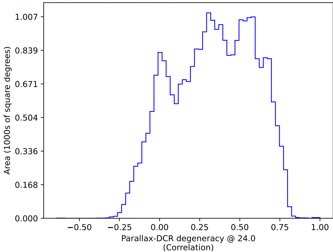
too_elab_2yr_r64_d2_ugrizy_v3.4_10yrs : Parallax-DCR degeneracy @ 24.0
