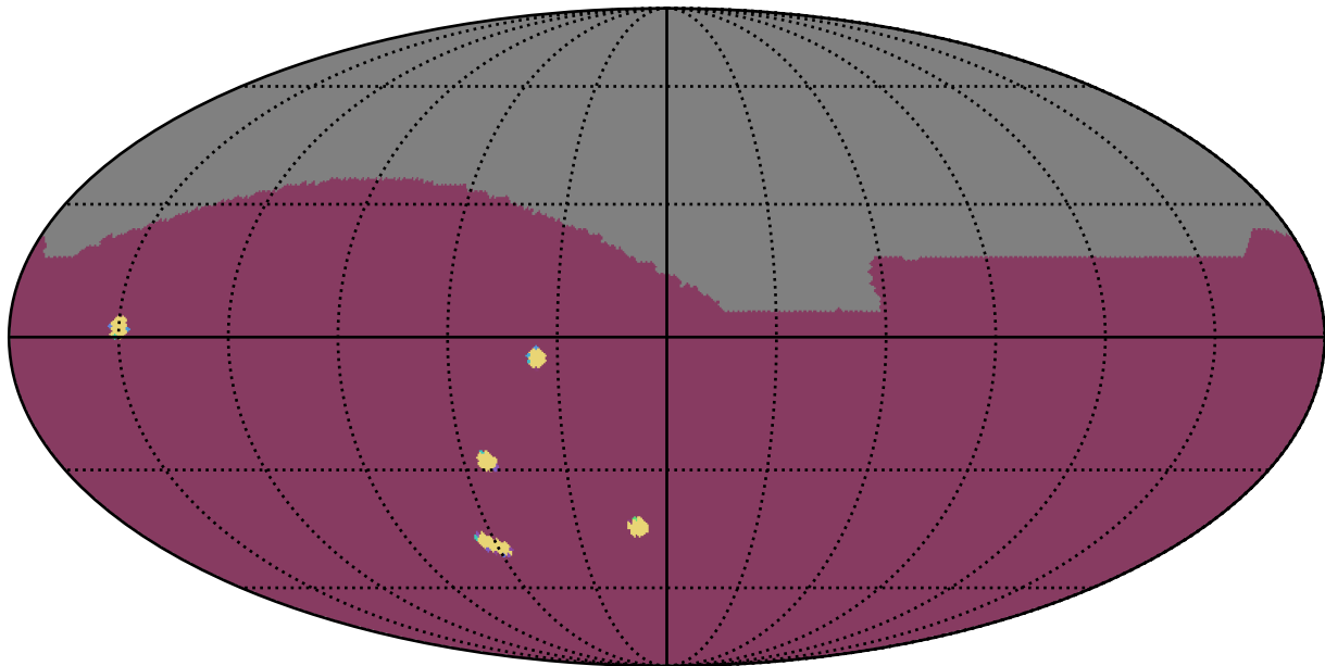
too_elab_2yr_r64_d2_ugrizy_v3.4_10yrs : NumberOfQuickRevisits
