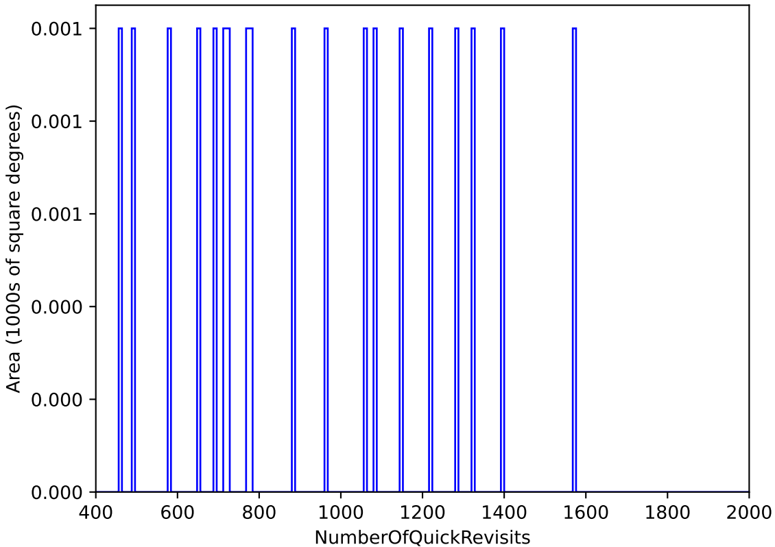
too_elab_2yr_r64_d2_ugrizy_v3.4_10yrs : NumberOfQuickRevisits
