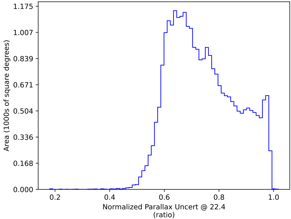
too_elab_2yr_r64_d2_ugrizy_v3.4_10yrs : Normalized Parallax Uncert @ 22.4
