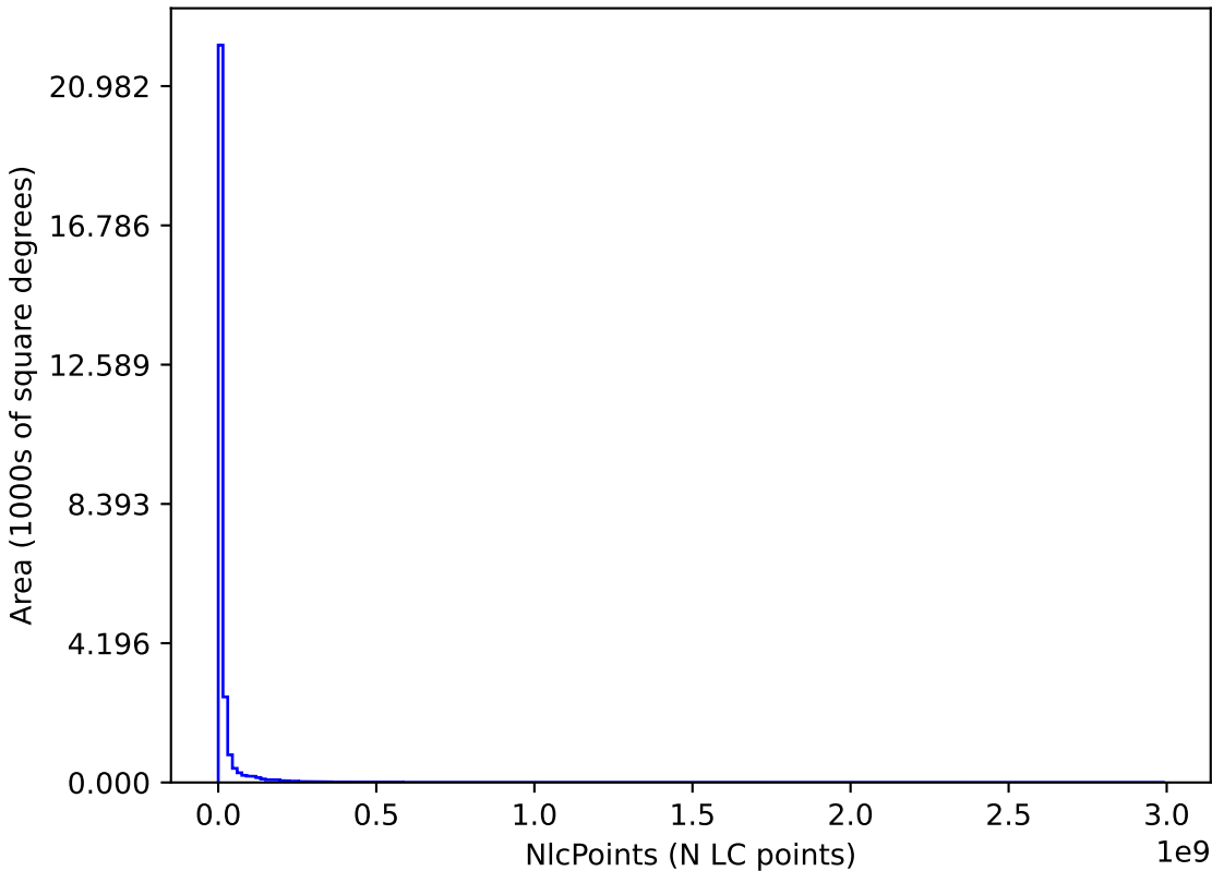
too_elab_2yr_r64_d2_ugrizy_v3.4_10yrs : NlcPoints
