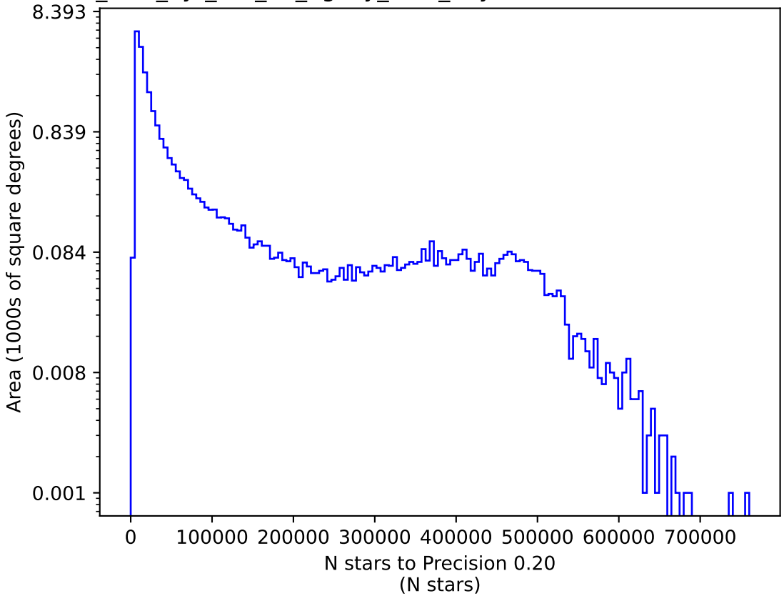
too_elab_2yr_r64_d2_ugrizy_v3.4_10yrs i: N stars to Precision 0.20
