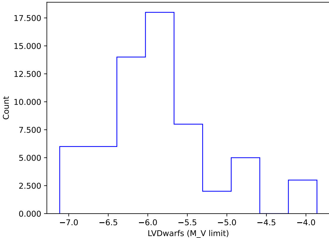
too_elab_2yr_r64_d2_ugrizy_v3.4_10yrs gi: LVDwarfs
