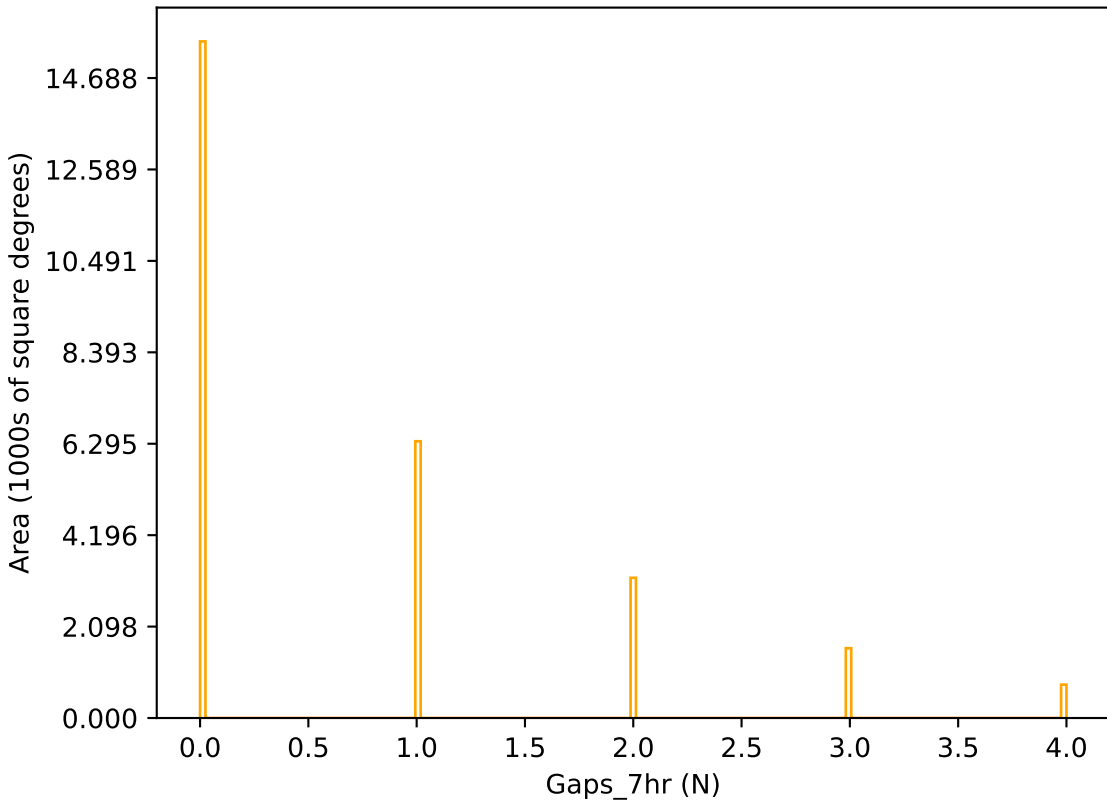
too_elab_2yr_r64_d2_ugrizy_v3.4_10yrs r band: Gaps_7hr
