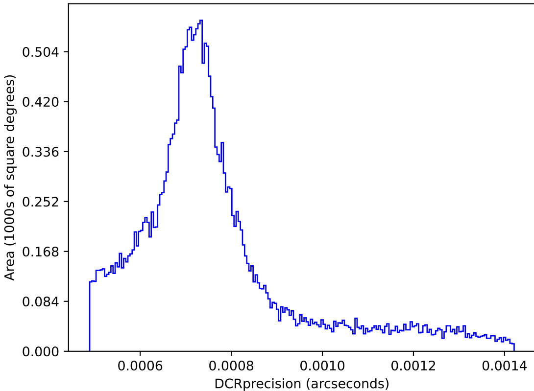
too_elab_2yr_r64_d2_ugrizy_v3.4_10yrs : DCRprecision
