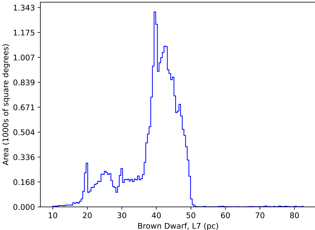
too_elab_2yr_r64_d2_ugrizy_v3.4_10yrs : Brown Dwarf, L7
