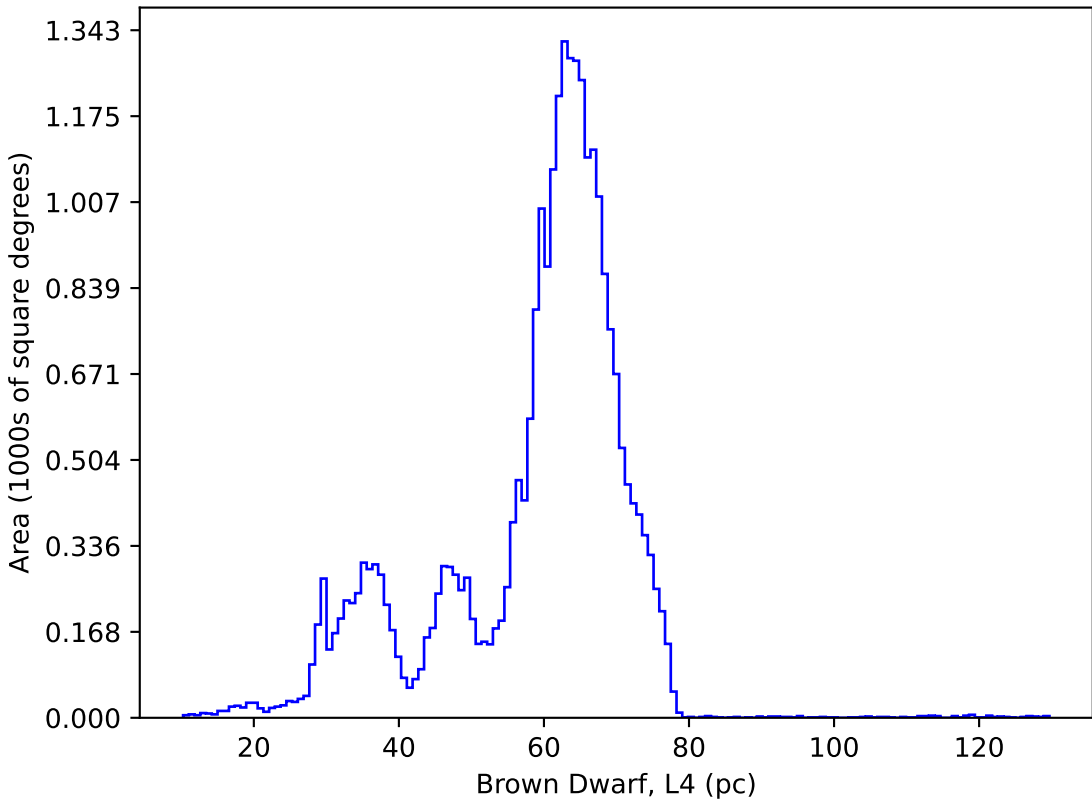
too_elab_2yr_r64_d2_ugrizy_v3.4_10yrs : Brown Dwarf, L4
