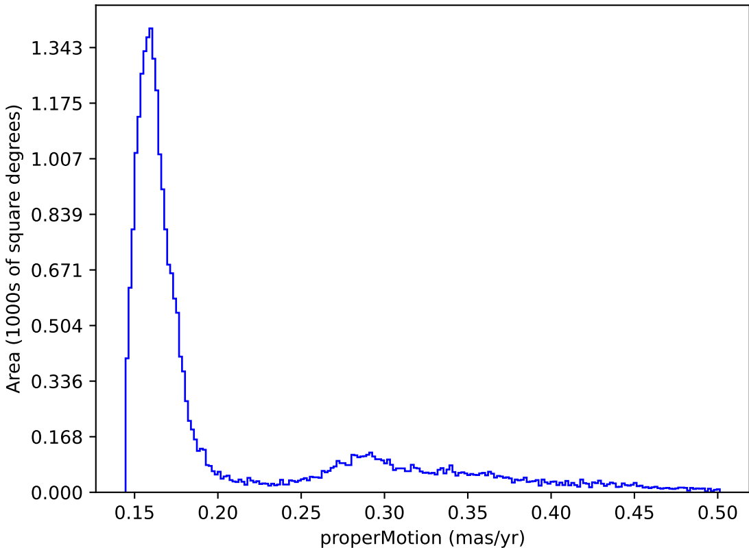
too_elab_2yr_r64_d2_ugrizy_v3.4_10yrs : properMotion
