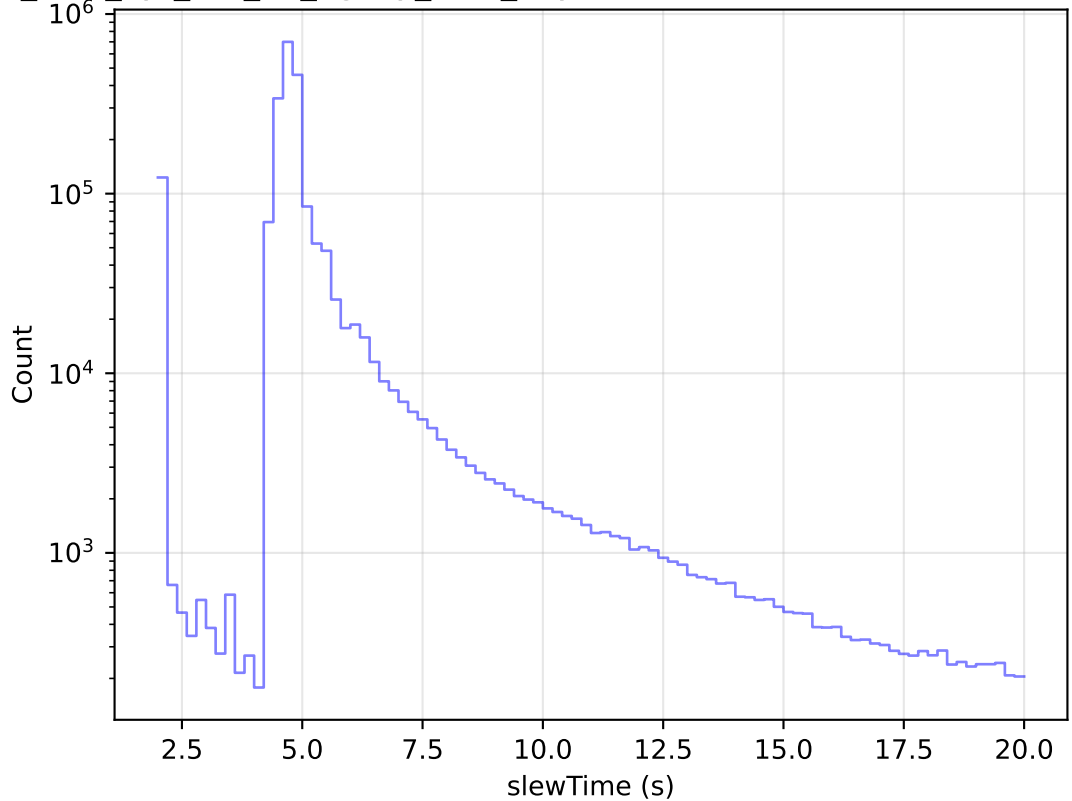
too_elab_2yr_r64_d2_ugrizy_v3.4_10yrs All visits: Zoom Slew Time Histogram
