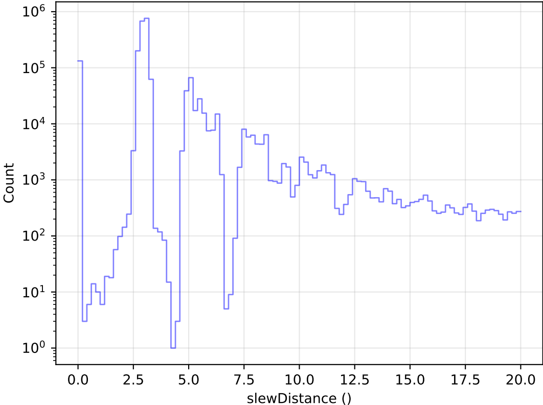
too_elab_2yr_r64_d2_ugrizy_v3.4_10yrs All visits: Zoom Slew Distance Histogram
