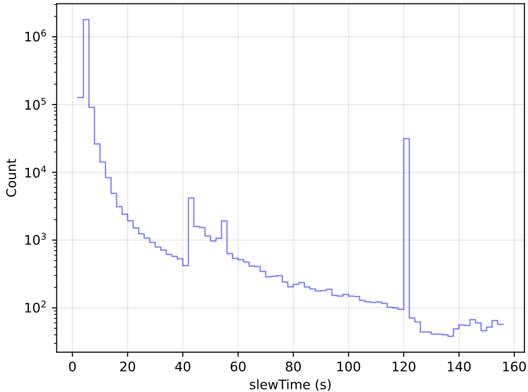
too_elab_2yr_r64_d2_ugrizy_v3.4_10yrs All visits: Slew Time Histogram
