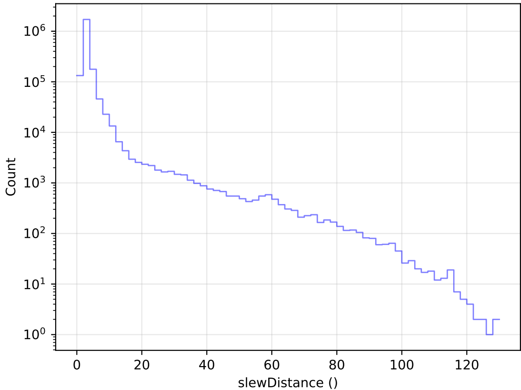
too_elab_2yr_r64_d2_ugrizy_v3.4_10yrs All visits: Slew Distance Histogram
