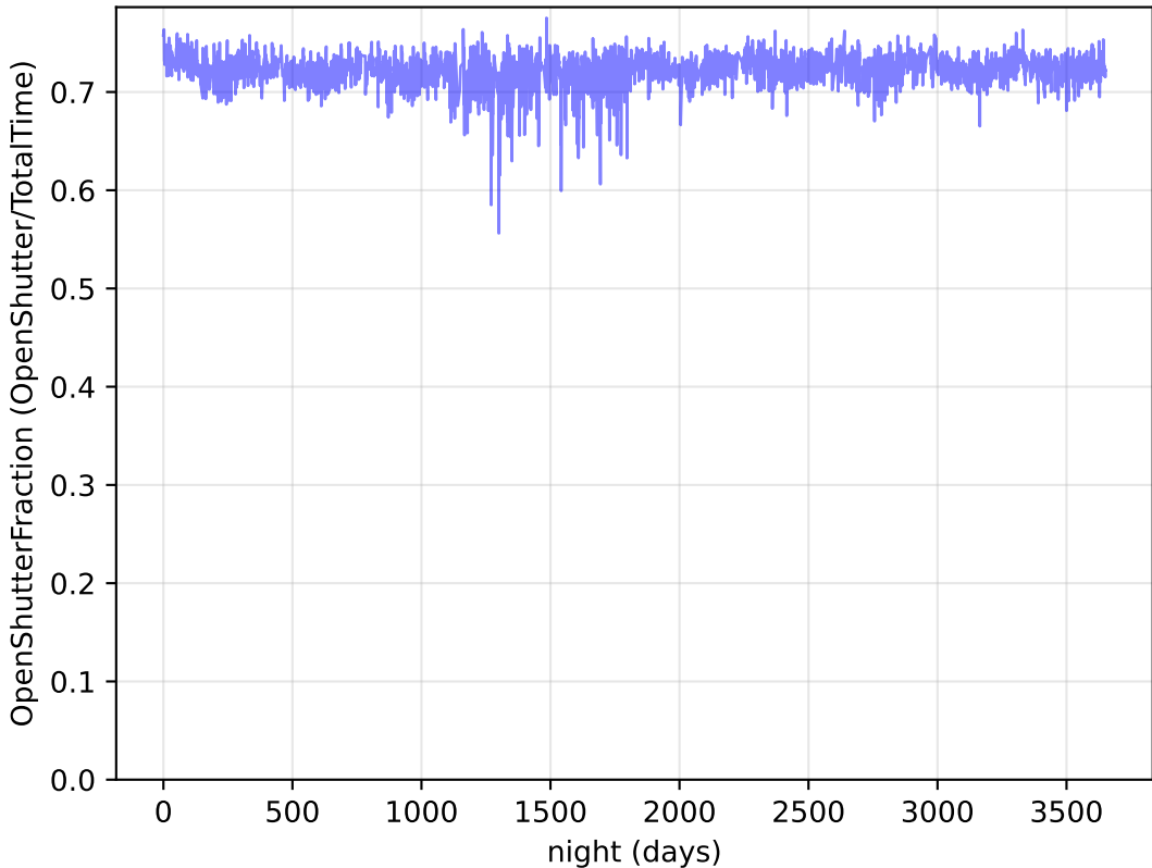
too_elab_2yr_r64_d2_ugrizy_v3.4_10yrs : OpenShutterFraction
