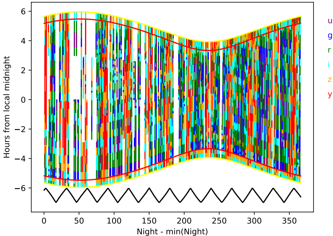
too_elab_2yr_r64_d2_ugrizy_v3.4_10yrs year 9-10: Hourglass
