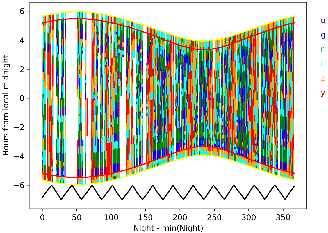
too_elab_2yr_r64_d2_ugrizy_v3.4_10yrs year 8-9: Hourglass
