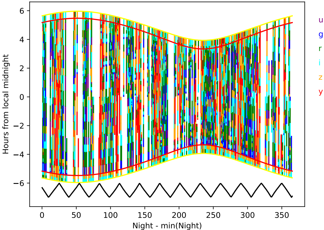
too_elab_2yr_r64_d2_ugrizy_v3.4_10yrs year 7-8: Hourglass
