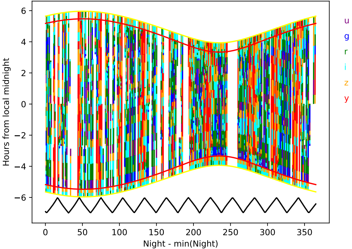
too_elab_2yr_r64_d2_ugrizy_v3.4_10yrs year 5-6: Hourglass
