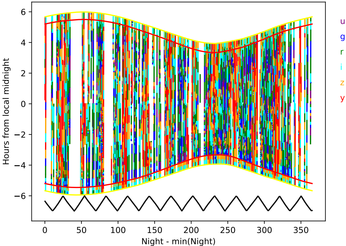
too_elab_2yr_r64_d2_ugrizy_v3.4_10yrs year 4-5: Hourglass
