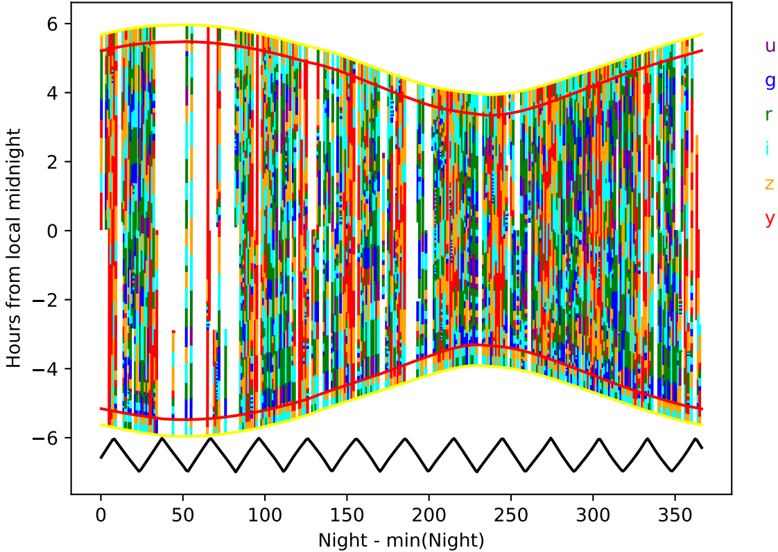
too_elab_2yr_r64_d2_ugrizy_v3.4_10yrs year 3-4: Hourglass
