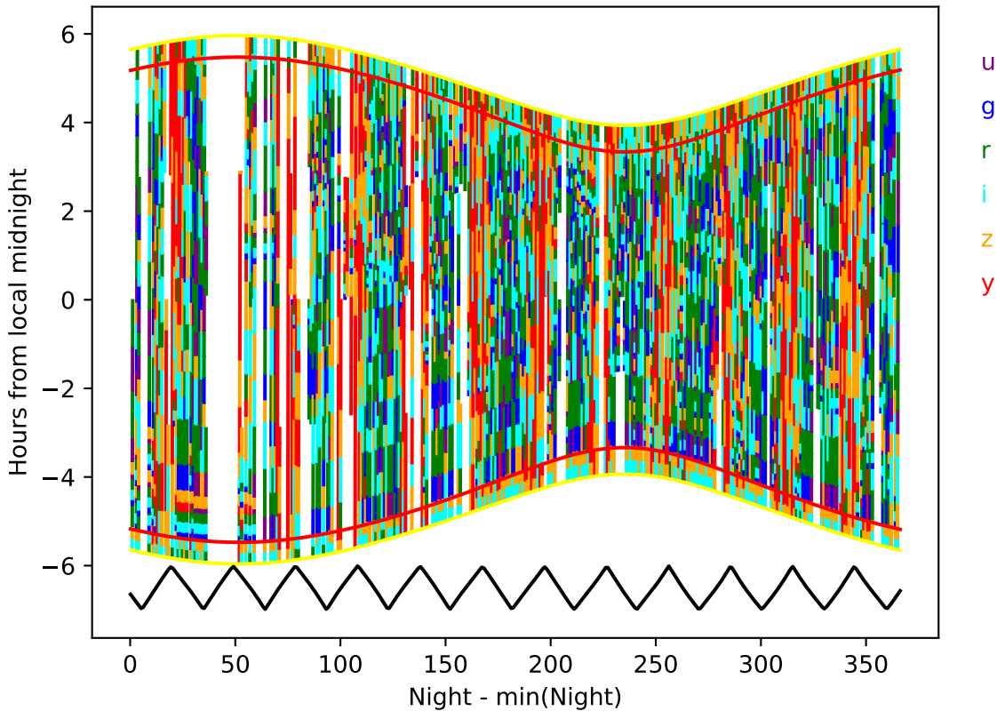
too_elab_2yr_r64_d2_ugrizy_v3.4_10yrs year 2-3: Hourglass
