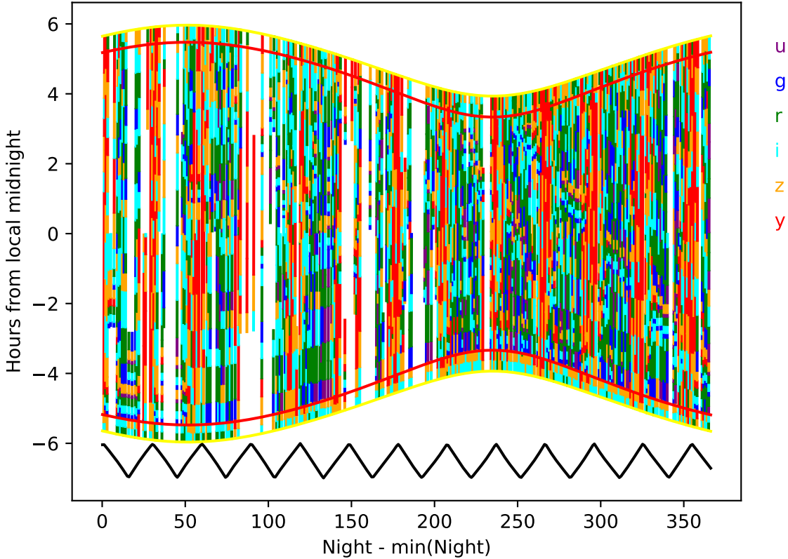
too_elab_2yr_r64_d2_ugrizy_v3.4_10yrs year 1-2: Hourglass
