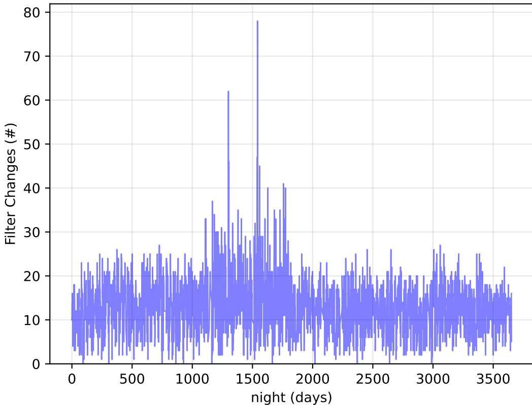
too_elab_2yr_r64_d2_ugrizy_v3.4_10yrs : Filter Changes
