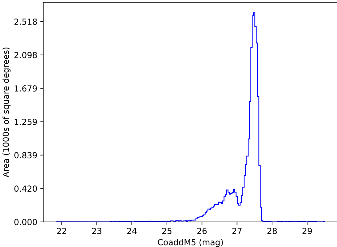
too_elab_2yr_r64_d2_ugrizy_v3.4_10yrs : CoaddM5
