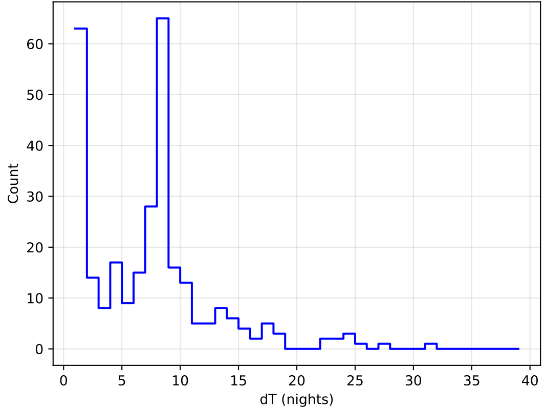
too_elab_2yr_r64_d2_ugrizy_v3.4_10yrs all bands: DD:XMM_LSS Delta Nights Histogram
