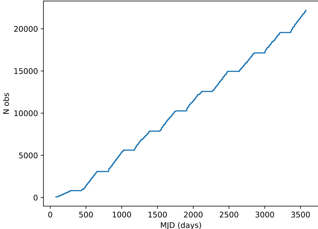
too_elab_2yr_r64_d2_ugrizy_v3.4_10yrs all bands: DD:XMM_LSS Cumulative NVisits
