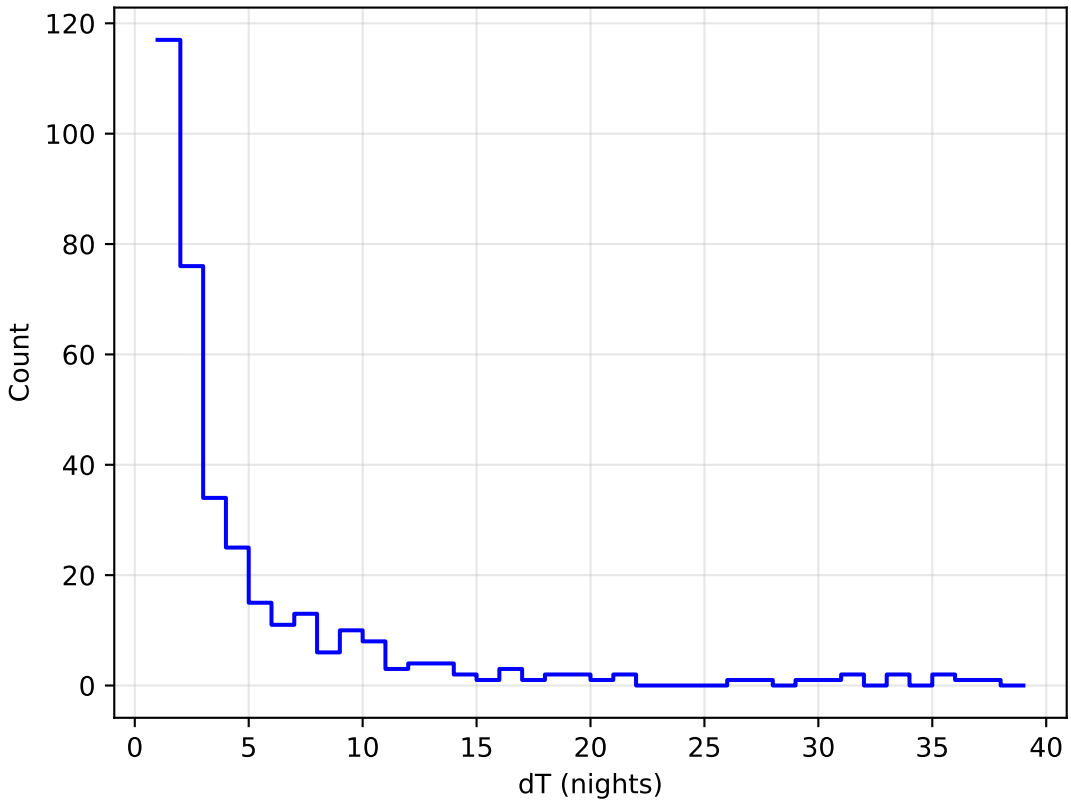
too_elab_2yr_r64_d2_ugrizy_v3.4_10yrs all bands: DD:WFD Delta Nights Histogram
