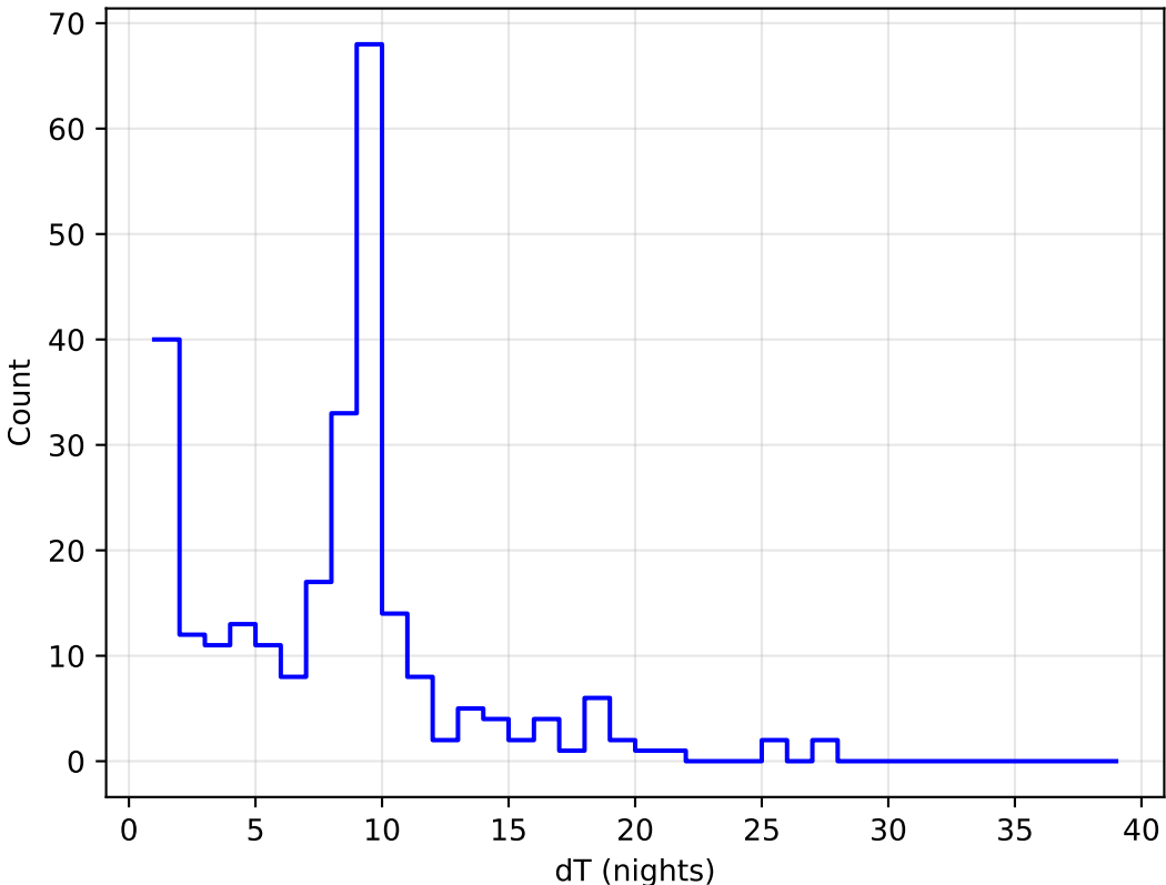
too_elab_2yr_r64_d2_ugrizy_v3.4_10yrs all bands: DD:ELAISS1 Delta Nights Histogram
