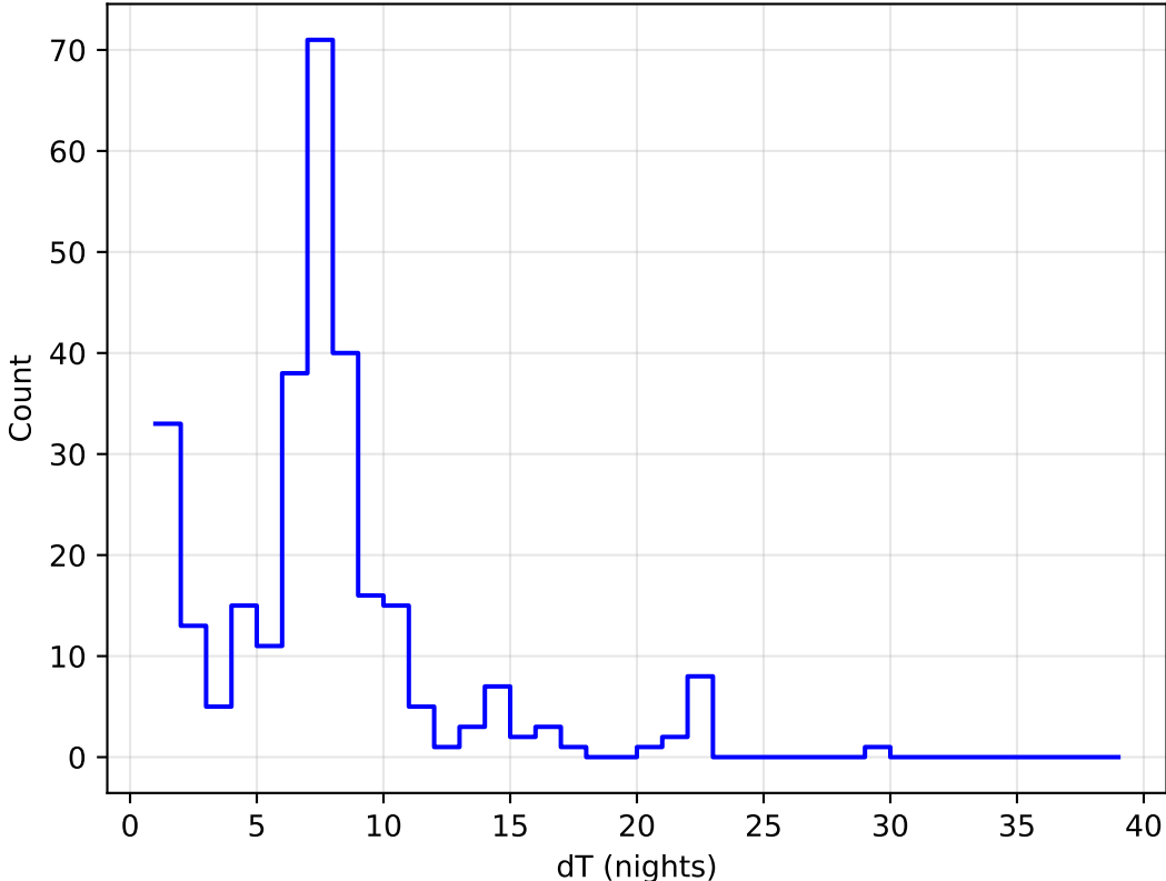
too_elab_2yr_r64_d2_ugrizy_v3.4_10yrs all bands: DD:EDFS Delta Nights Histogram
